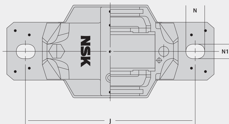
PILLOW BLOCK DIMENSIONS
