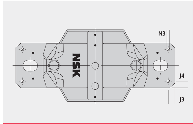
RECOMMENDED DIMENSIONS: LOCATING PIN HOLES (MM)
