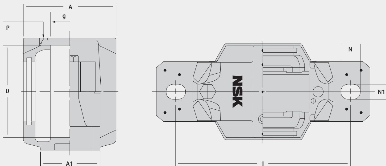
PILLOW BLOCK DIMENSIONS
