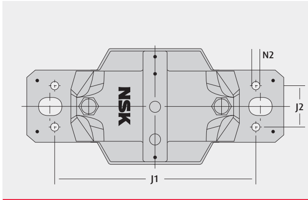
RECOMMENDED DIMENSIONS: 4 BOLT FIXING HOLES (MM)
